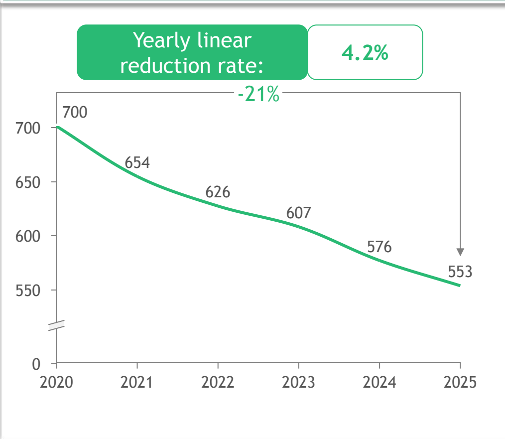
Shengmu GHG Emission Projection (k ton CO 2 e, 2020-2025E)
