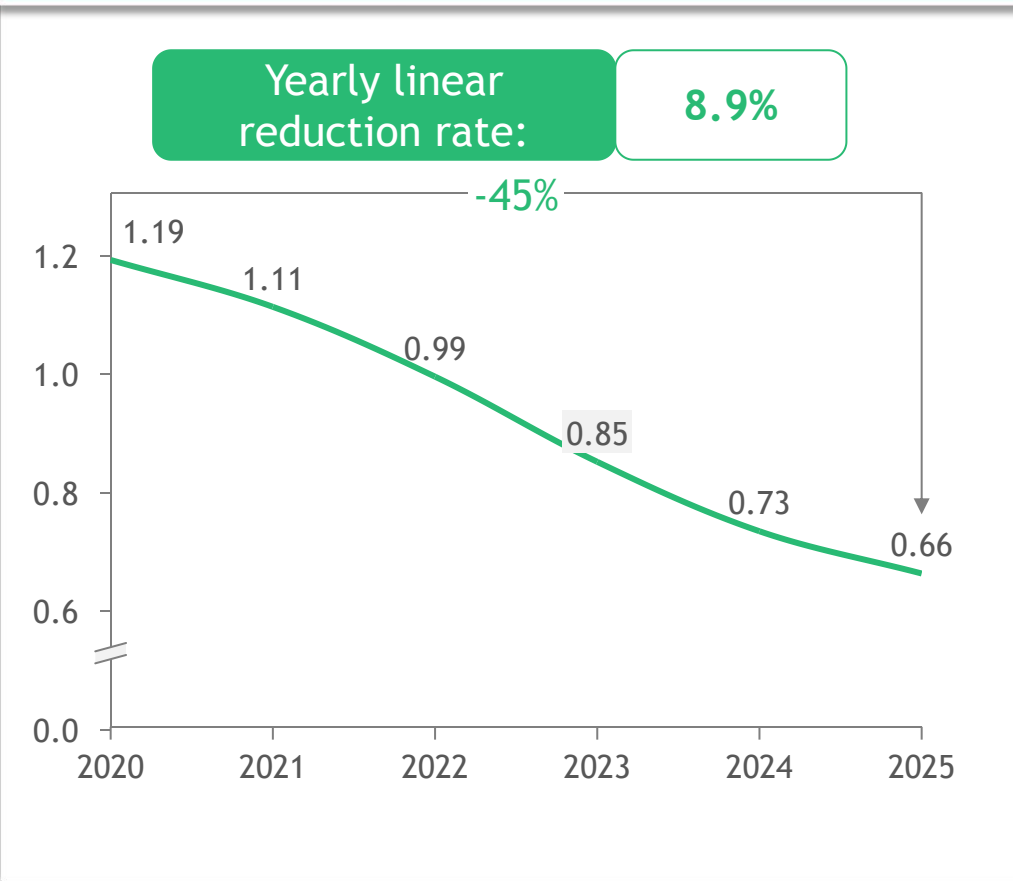
Shengmu GHG Emission Intensity Projection (kg CO 2 e/kg FPCM, 2020-2025E)
